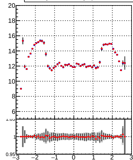
mean hit Legend: DQM_TT_mkFit-DQM_pless_orig (blue line), DQM_TT_mkFit-DQM_pless_modi3 (red line)
