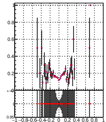
—●— DQM_TT_mkFit-DQM_pless_orig —●— DQM_TT_mkFit-DQM_pless_modi3
