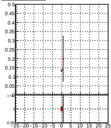
—●— DQM_TT_mkFit-DQM_pless_orig —●— DQM_TT_mkFit-DQM_pless_modi3
