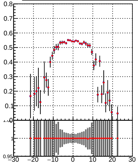
Efficiency vs. sim PV z Legend: DQM_TT_mkFit-DQM_pless_orig (blue line) DQM_TT_mkFit-DQM_pless_modi3 (red line)
