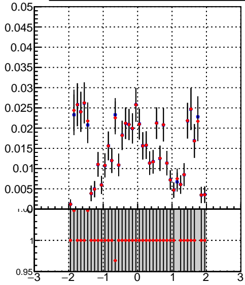
■ DQM_TT_mkFit-DQM_pless_orig ● DQM_TT_mkFit-DQM_pless_modi3
