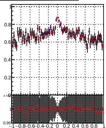
DQM_TT_mkFit-DQM_pless_modi3
