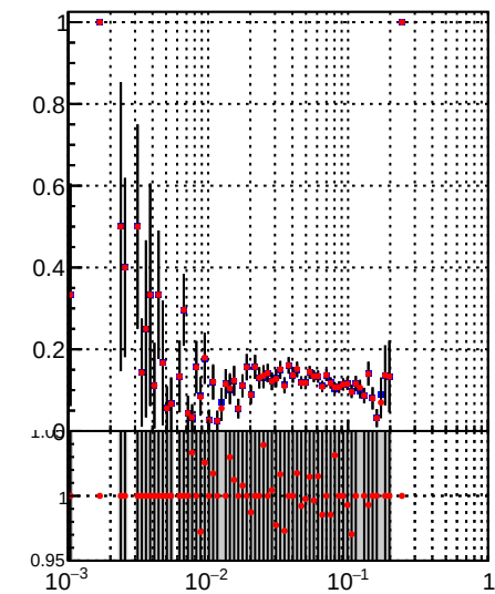
Fake rate vs \sqrt{s} Legend: —•— DQM_TT_mkFit-DQM_pless_orig —•— DQM_TT_mkFit-DQM_pless_modi3
