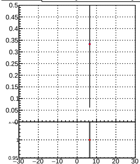
Fake rate vs vertpos Legend: DQM_TT_mkFit-DQM_pless_orig (grey shaded region) DQM_TT_mkFit-DQM_pless_modi3 (red dot with error bar)
