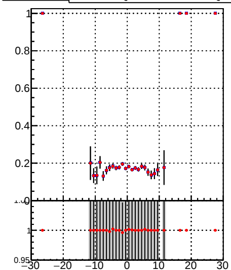
—•— DQM_TT_mkFit-DQM_pless_orig —•— DQM_TT_mkFit-DQM_pless_modi3
