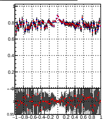
DQM_TT_mkFit-DQM_pless_modi3
