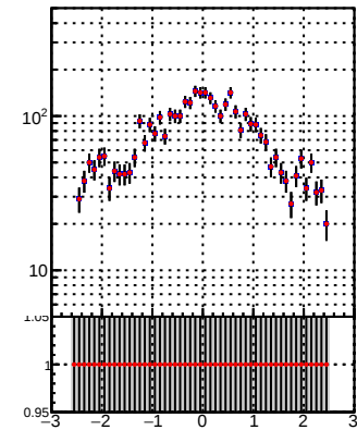
N of reco track vs \eta pT eta Legend: DQM_TT_mkFit-DQM_pless_orig (black dots with error bars) DQM_TT_mkFit-DQM_pless_modi3 (red dots with error bars)
