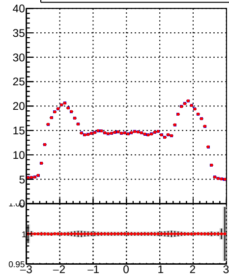
mean hit — DQM_TT_mkFit-DQM_pless_orig — DQM_TT_mkFit-DQM_pless_modi3
