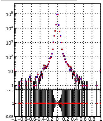
Legend: DQM_TT_mkFit-DQM_pless_orig (black line with dots) DQM_TT_mkFit-DQM_pless_modi3 (red line with dots)
