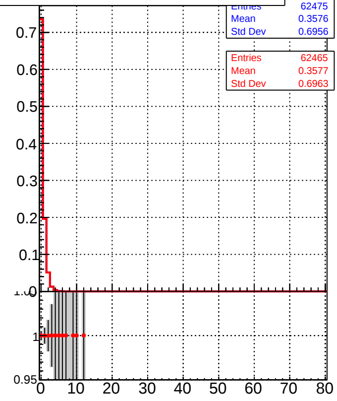
Legend for bottom row plots: DQM_TT_mkFit-DQM_pless_orig DQM_TT_mkFit-DQM_pless_modi3
