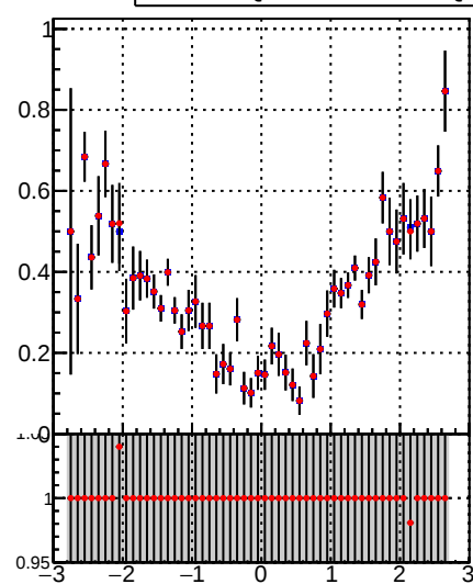
—•— DQM_TT_mkFit-DQM_pless_orig —•— DQM_TT_mkFit-DQM_pless_modi3
