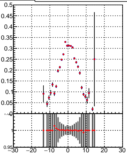
Fake rate vs v —■ DQM_TT_mkFit-DQM_pless_orig —◆ DQM_TT_mkFit-DQM_pless_modi3
