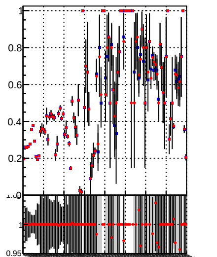
Fake rate vs. —●— DQM_TT_mkFit-DQM_pless_orig —●— DQM_TT_mkFit-DQM_pless_modi3
