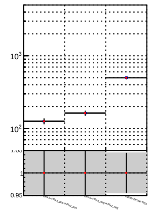
N of reco track vs. \chi^2 —•— DQM TT mkFit-DQM_pless_orig —•— DQM TT mkFit-DQM_pless_modi3
