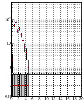
N of reco track vs. \chi^2 DQM TT mkFit-DQM_pless_orig DQM TT mkFit-DQM_pless_modi3
