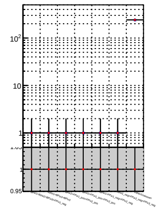
N of reco track vs. \chi^2 DQM TT mkFit-DQM_pless_orig DQM TT mkFit-DQM_pless_modi3
