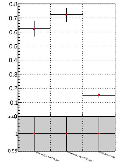
Fake rate vs. — DQM_TT_mkFit-DQM_pless_orig — DQM_TT_mkFit-DQM_pless_modi3
