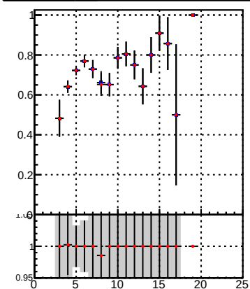
Fake rate vs hit Legend: DQM_TT_mkFit-DQM_pless_orig (grey histogram), DQM_TT_mkFit-DQM_pless_modi3 (red line with error bars)
