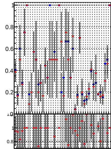
Fake rate vs. — DQM_TT_mkFit-DQM_pless_orig — DQM_TT_mkFit-DQM_pless_modi3
