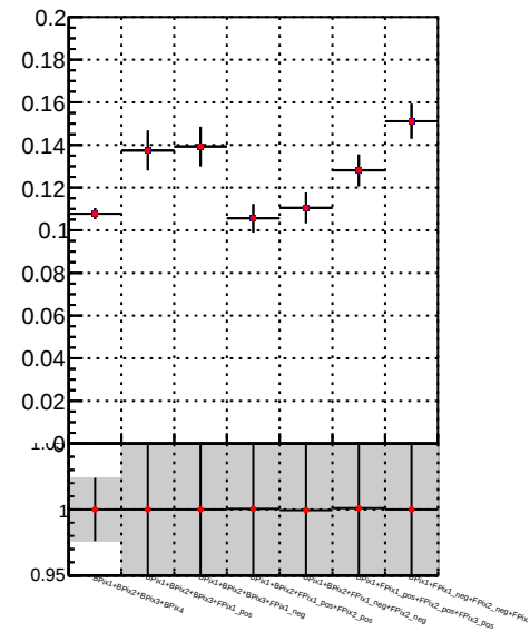
Fake rate vs. —•— DQM_TT_mkFit-DQM_pless_orig —•— DQM_TT_mkFit-DQM_pless_modi3
