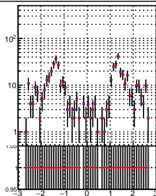
N of reco track vs \eta DQM_TT_mkFit-DQM_pless_orig DQM_TT_mkFit-DQM_pless_modi3
