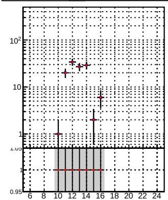
Legend: DQM_TT_mkFit-DQM_pless_orig (blue line with dots), DQM_TT_mkFit-DQM_pless_modi3 (red line with stars)
