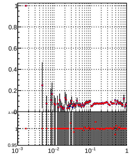
Fake rate vs \sqrt{s} Legend: DQM_TT_mkFit-DQM_pless_orig (blue line with error bars) DQM_TT_mkFit-DQM_pless_modi3 (red line with error bars)
