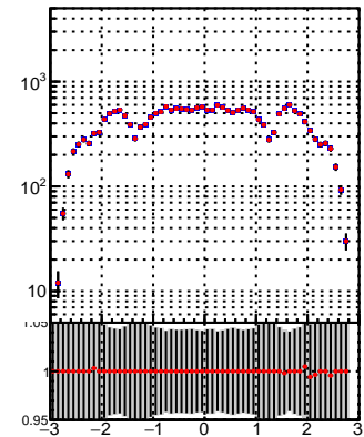
N of reco track vs \eta Legend: DQM_TT_mkFit-DQM_pless_orig (blue line with markers) DQM_TT_mkFit-DQM_pless_modi3 (red line with markers)
