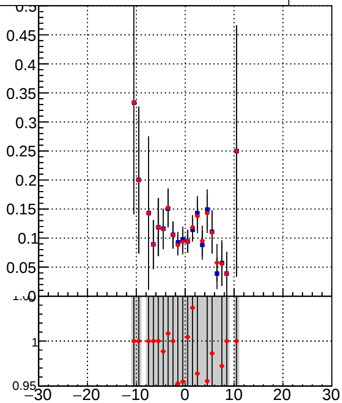
DQM_TT_mkFit-DQM_pless_orig DQM_TT_mkFit-DQM_pless_modi3
