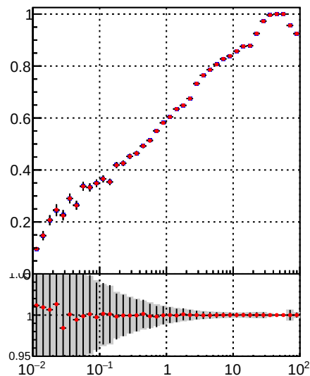
—•— DQM_TT_mkFit-DQM_pless_orig —•— DQM_TT_mkFit-DQM_pless_modi3
