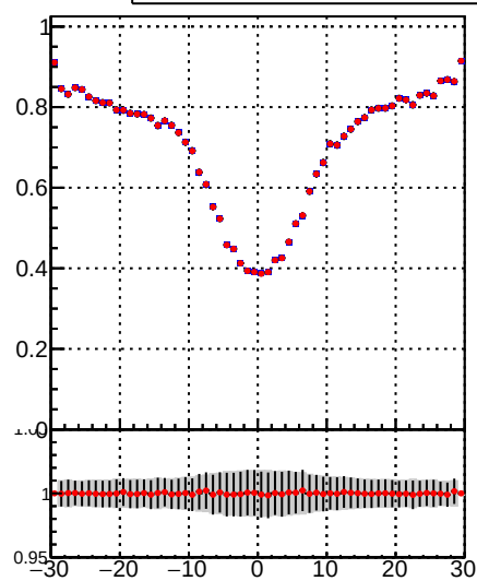
—•— DQM_TT_mkFit-DQM_pless_orig —•— DQM_TT_mkFit-DQM_pless_modi3
