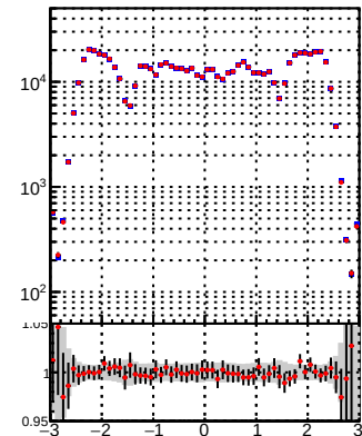
—•— DQM_TT_mkFit-DQM_pless_orig —•— DQM_TT_mkFit-DQM_pless_modi3
