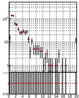
N of reco track vs. \chi^2 — DQM TT mkFit-DQM_pless_orig — DQM TT mkFit-DQM_pless_mod13
