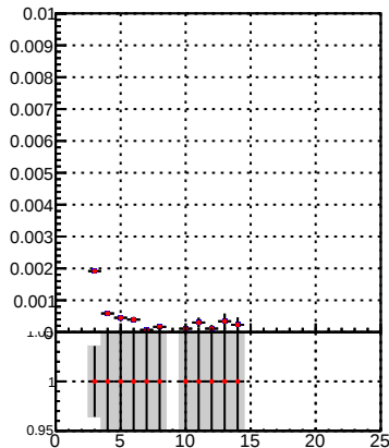
DQM_TT_mkFit-DQM_pless_modi3
