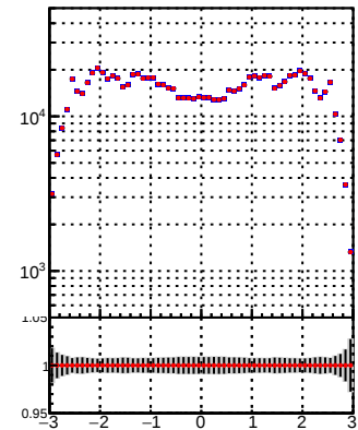
N of reco track vs \eta Legend: DQM_TT_mkFit-DQM_pless_orig (blue line with dots) DQM_TT_mkFit-DQM_pless_modi3 (red line with dots)
