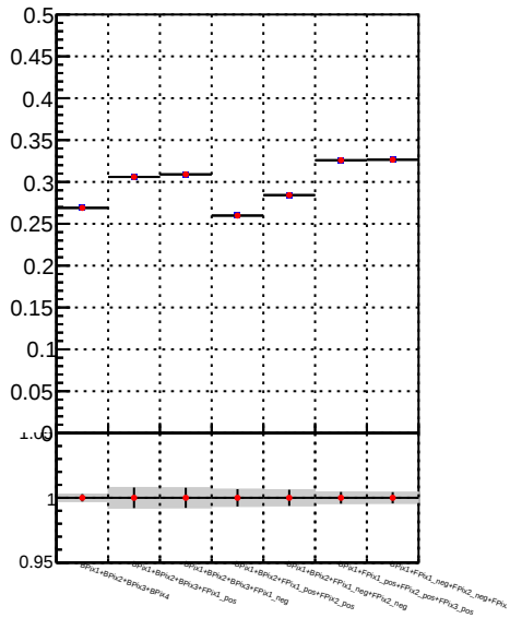
Fake rate vs. DQM TT mkFit-DQM_pless_orig DQM TT mkFit-DQM_pless_modi3
