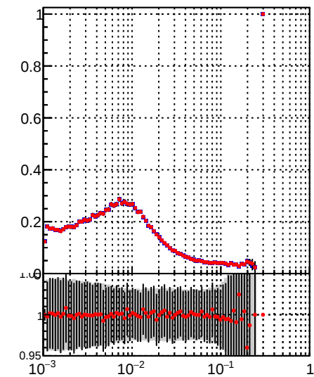
—•— DQM_TT_mkFit-DQM_pless_orig —•— DQM_TT_mkFit-DQM_pless_modi3
