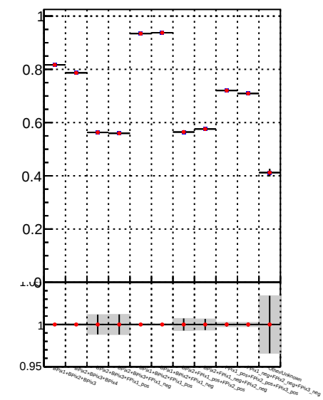
Fake rate vs. — DQM TT_mkFit-DQM_pless_orig — DQM TT_mkFit-DQM_pless_modi3
