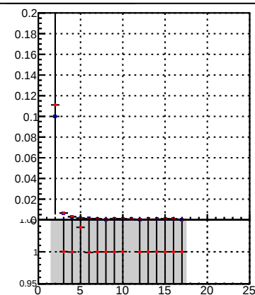
DQM_TT_mkFit-DQM_pless_orig
