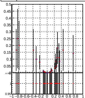
Efficienc — DQM_TT_mkFit-DQM_pless_modi3
