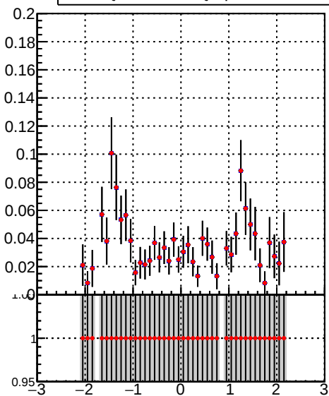
■ DQM_TT_mkFit-DQM_pless_orig ● DQM_TT_mkFit-DQM_pless_modi3
