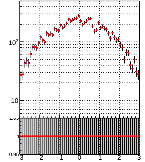
N of simulated tracks vs phi Legend: DQM_TT_mkFit-DQM_pless_orig (grey line) DQM_TT_mkFit-DQM_pless_modi3 (red line)
