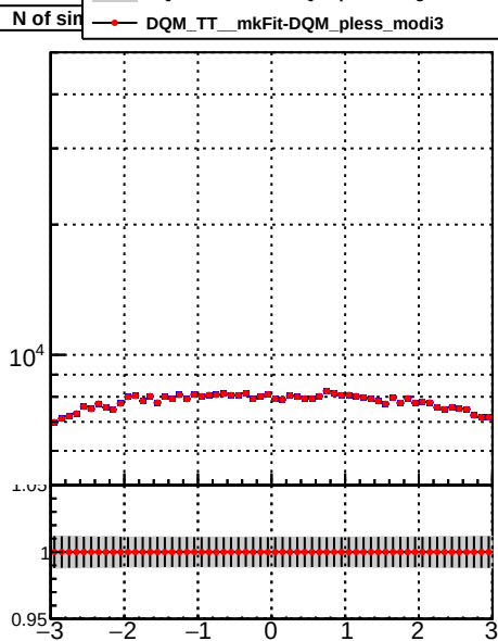
N of simulated tracks vs phi
