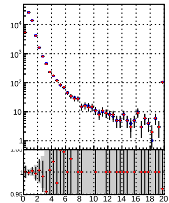
N of reco track vs. DQM_TT mkFit-DQM_pless_orig DQM_TT mkFit-DQM_pless_modi3
