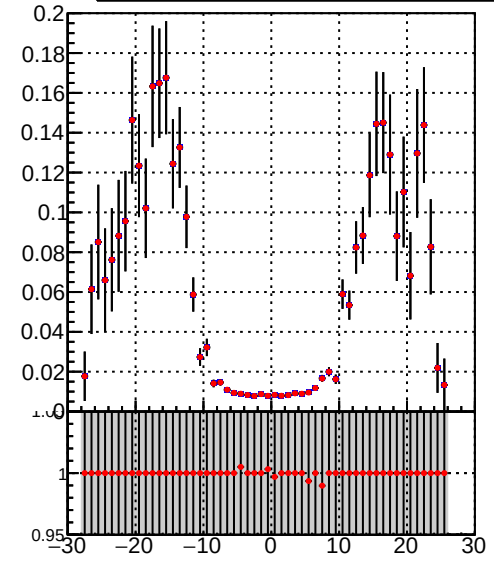
Efficiency vs. sim PV z Legend: DQM_TT_mkFit-DQM_pless_orig (blue line with error bars) DQM_TT_mkFit-DQM_pless_modi3 (red line with error bars)
