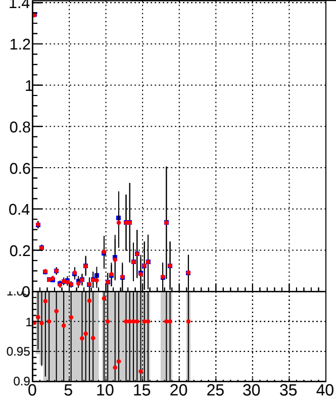
K_S^0 tracking fake rate vs p_T Legend: \blacksquare DQM_TT_mkFit-DQM_pless_orig \bullet DQM_TT_mkFit-DQM_pless_modi3
