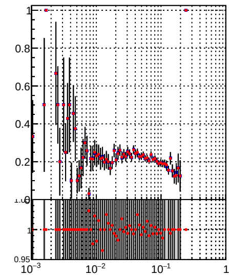
Fake rate vs \sqrt{s} DQM_TT_mkFit-DQM_pless_orig DQM_TT_mkFit-DQM_pless_modi3
