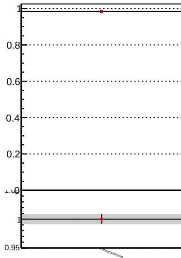
Fake rate vs. — DQM TT mkFit-DQM_pless_orig — DQM TT mkFit-DQM_pless_modi3
