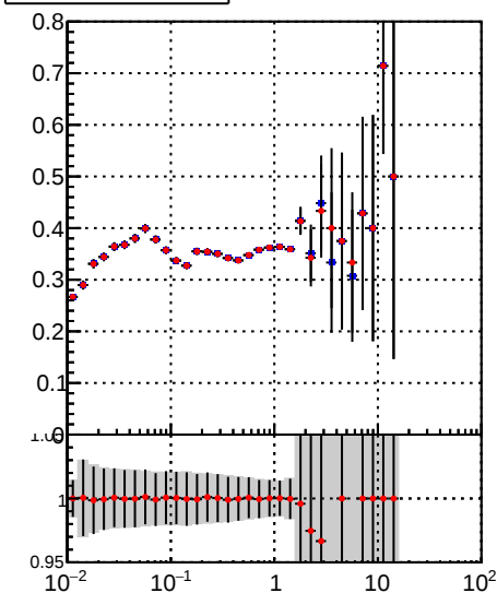
—•— DQM_TT_mkFit-DQM_pless_orig —•— DQM_TT_mkFit-DQM_pless_modi3
