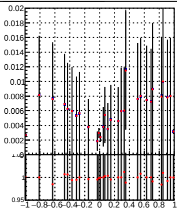
DQM_TT_mkFit-DQM_pless_orig
