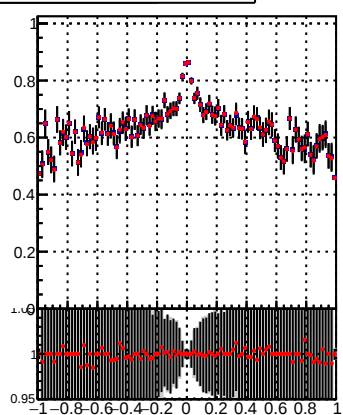
DQM_TT_mkFit-DQM_pless_modi3
