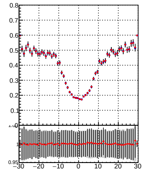
—•— DQM_TT_mkFit-DQM_pless_orig —•— DQM_TT_mkFit-DQM_pless_modi3
