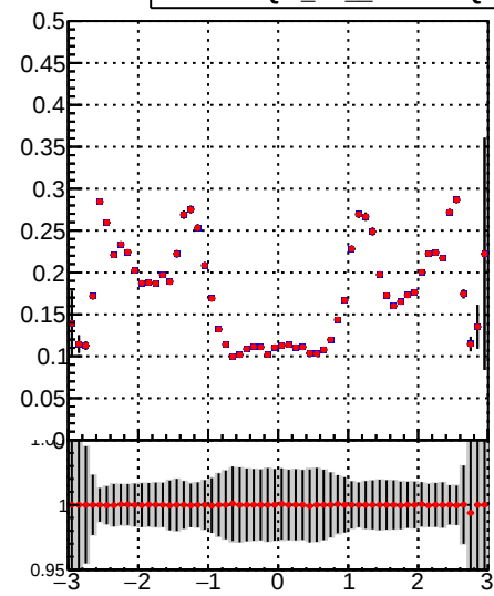
—•— DQM_TT_mkFit-DQM_pless_orig —•— DQM_TT_mkFit-DQM_pless_modi3
