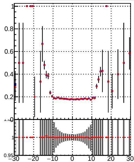
—•— DQM_TT_mkFit-DQM_pless_orig —•— DQM_TT_mkFit-DQM_pless_modi3
